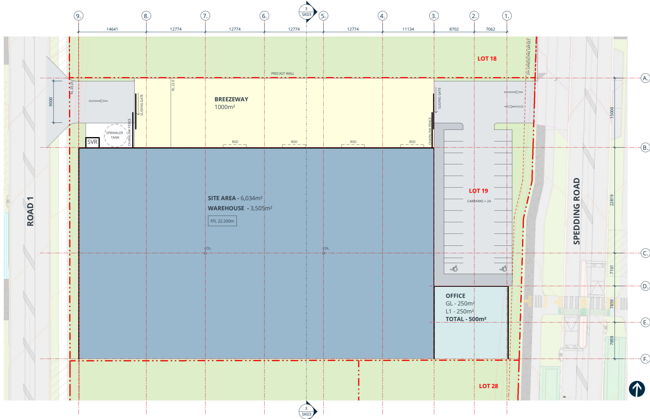
1 SITE PLAN - B&L - LOT 19 SCALE @ A1: 1 : 250
